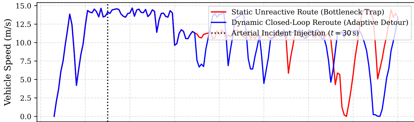
(a) Real-Time Vehicle Speed Profile in SUMO Simulation
