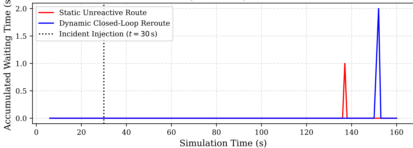
(b) Queue Waiting Time Delay Behind Bottleneck
